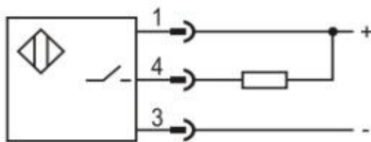
NPN NO
