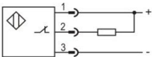
NPN NC
