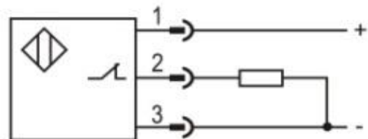
PNP NC
